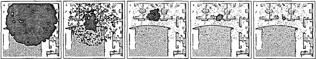
Fig. 6. Evolution of the posterior about the localization of an RFID tag over time. The width of the circles represents the importance weight of the corresponding particle. It is drawn proportional to the ratio between the importance weights of the particular sample and the maximum likelihood sample.
