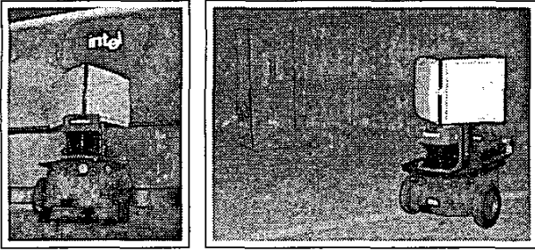
Fig. 2. Pioneer 2 with Sick Laser Range Finder, RFID reader and two antennas (left). Experimental setup used for learning the likelihood function of tag detections (right).
